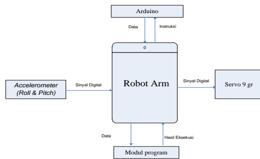
Gambar 6. Context Diagram
