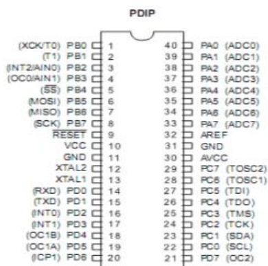
Gambar 2. Kofigurasi PIN ATmega16
