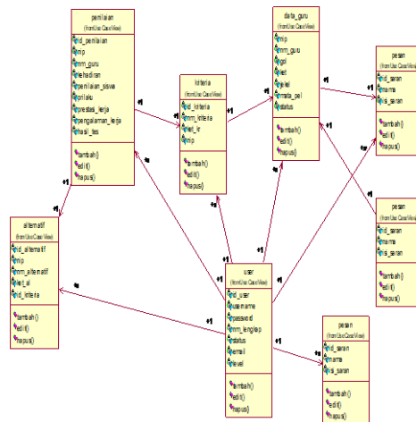
Gambar 5. Class Diagram System
