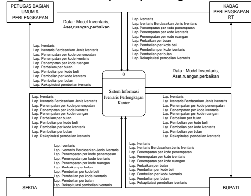
Gambar 3. Context Diagram
